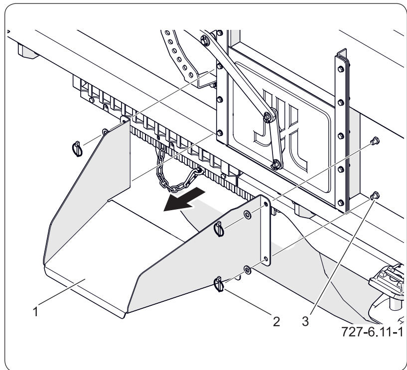
Figure 6.24 Goulotte
