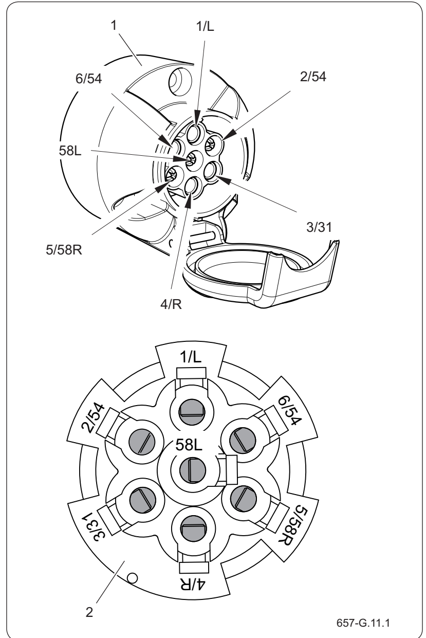
Figure 4.11 Prise 7 broches
