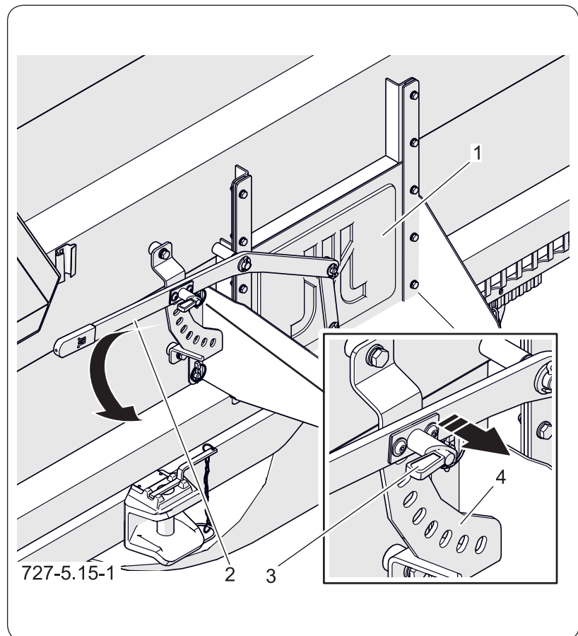
Figure 5.21 Goulotte
